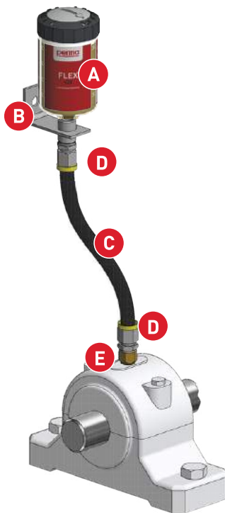
Installation example roller bearing lubrication
